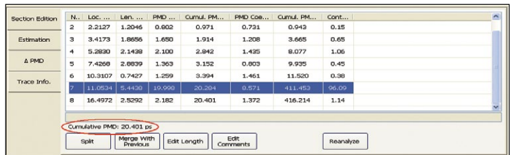
Before fixing the faulty 5 km fiber span (section 8).
