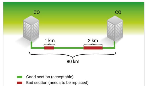
Contrary to the traditional approach, distributed PMD analysis breaks down the measurement results, effectively pinpointing the high-contributing sections of the link.
