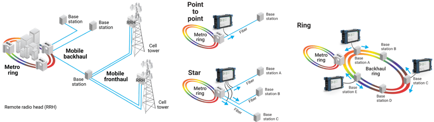
Mobile backhaul
