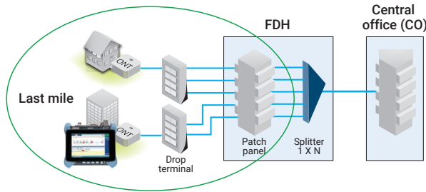
Figure 1. Certification of last-mile FTTx including continuity at splitter.
