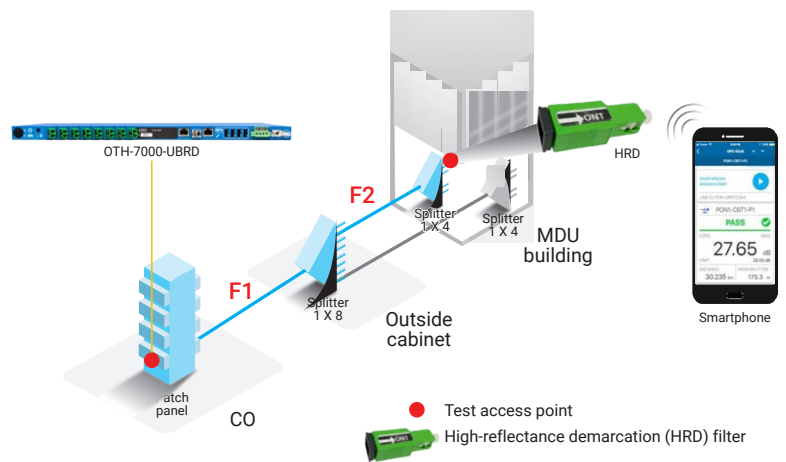
Link certification in a PON architecture with end-to-end connectivity.
