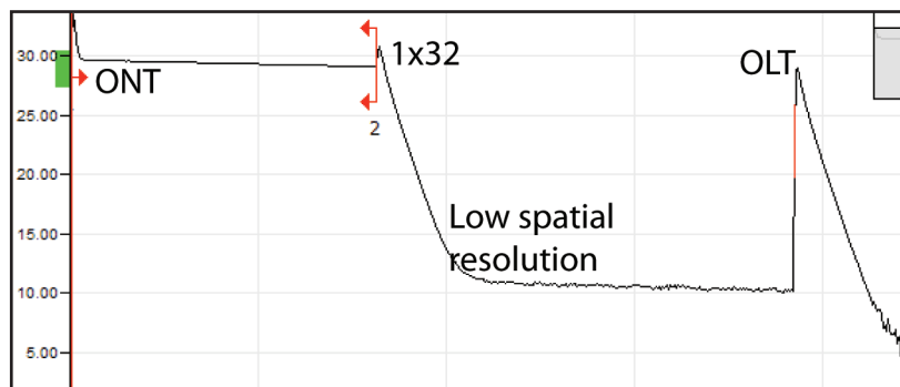
Figure 1 (a), (b), (c): OTDR trace examples after the 1x32 splitter with a PON OTDR that is not optimized
