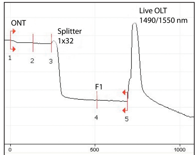
Figure 2: PON-optimized OTDR trace from the ONT to the OLT splitter
