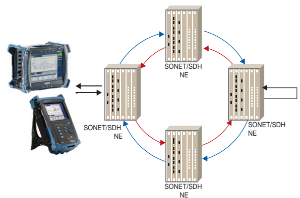
Housed in the FTB-500 or FTB-200 platform, the FTB-8120/8130 modules offer the solution for field circuit turn-up and troubleshooting.
