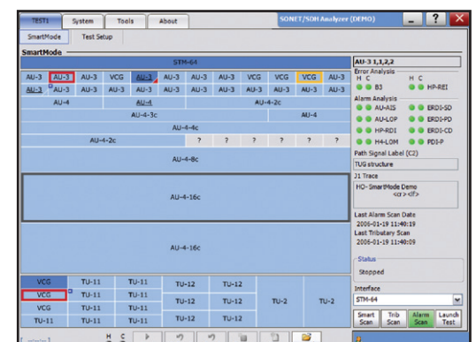
FTB-8120/8130 SmartMode: multichannel signal discovery with real-time alarm scan (shown in the FTB-500 user interface).
