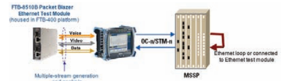
Combining the FTB-8510B's Ethernet multiple-streaming capabilities and the FTB-8120NG/8130NG embedded Ethernet interfaces creates a powerful solution for testing multiple services over SONET/SDH.
