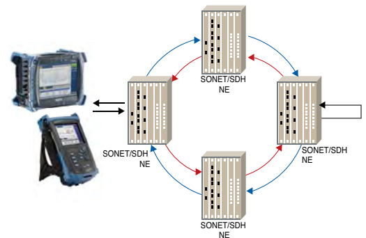
Housed in either the FTB-500 or FTB-200 platform, the FTB-8120NGE/8130NGE modules offer the solution for field circuit turn-up and troubleshooting.
