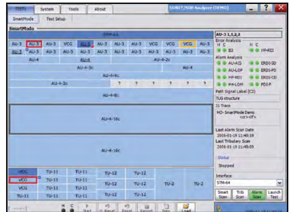
FTB-8120NGE/8130NGE SmartMode: multichannel signal discovery with real-time alarm scan (shown in the FTB-500 user interface).
